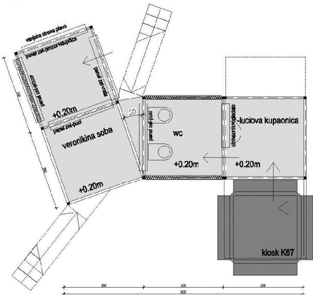
_groundfloor +0.20
